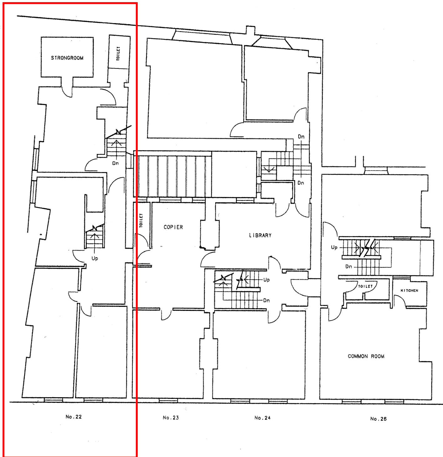
FIRST FLOOR PLAN - GUILDHALL CHAMBERS
